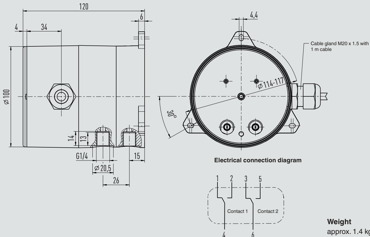
Model DPS40 with aluminium measuring chamber, 2 x G 1/4 female thread, centre distance 26 mm
