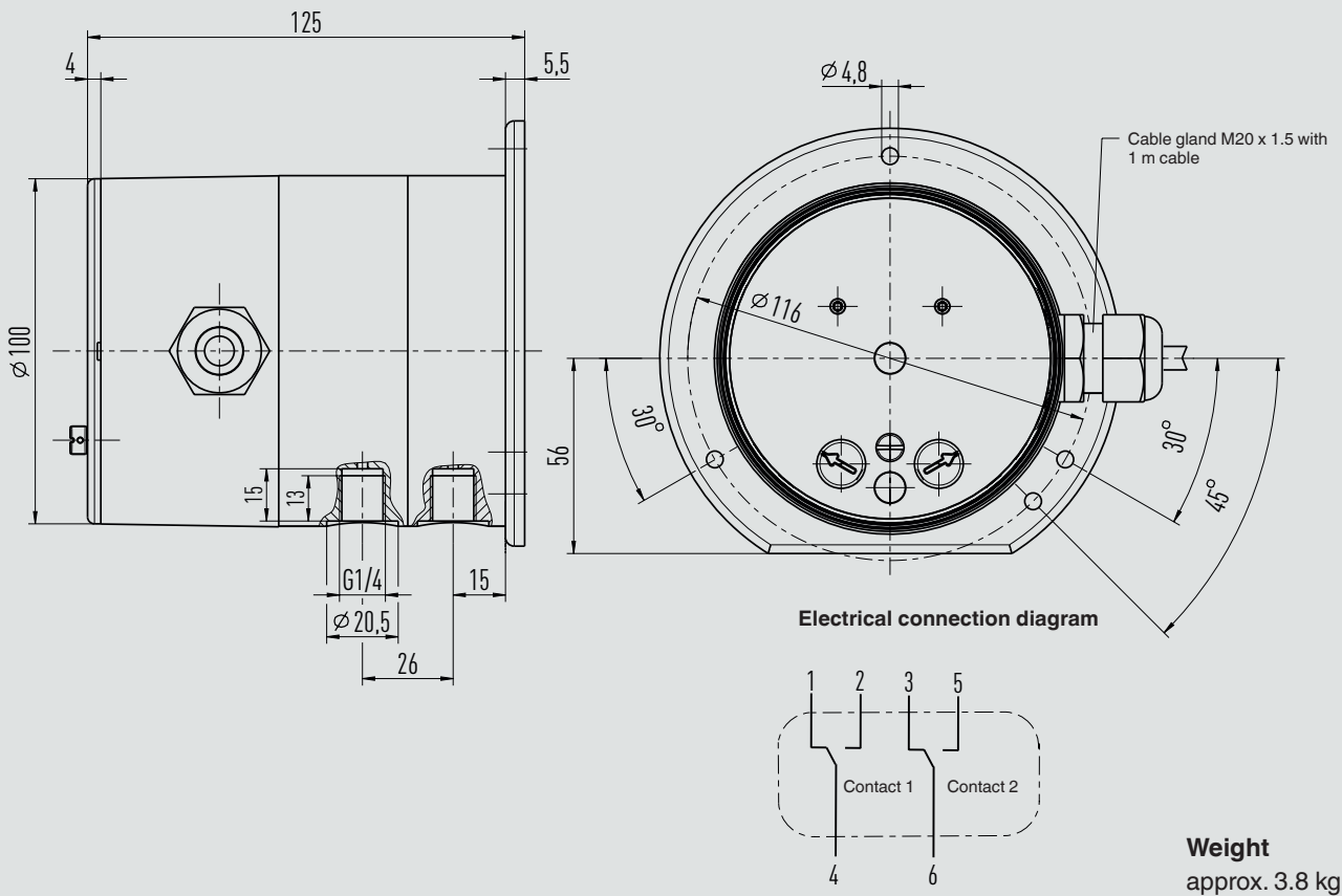
Model DPS40 with stainless steel measuring chamber, 2 x G 1/4 female thread, centre distance 26 mm
